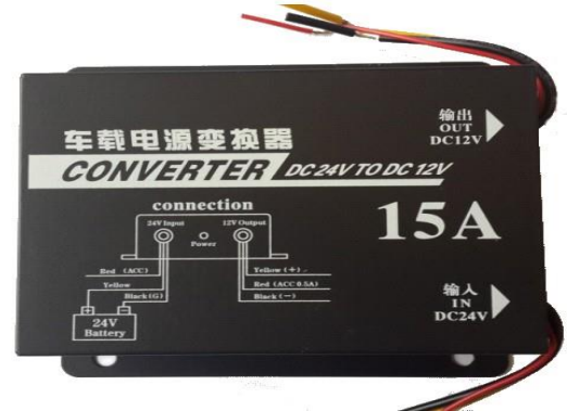
CONVERTER REG15/2 24 TO 12V STEP DOWN BOX 15AMP
